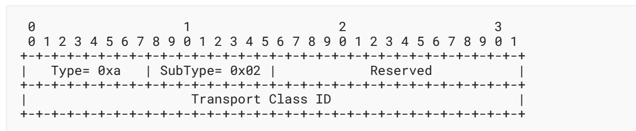
Figure 2: Transport Class RT
