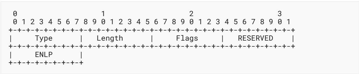
Figure 15: ENLP Sub-TLV
